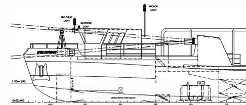
PORT SIDE PROFILE (PART)
