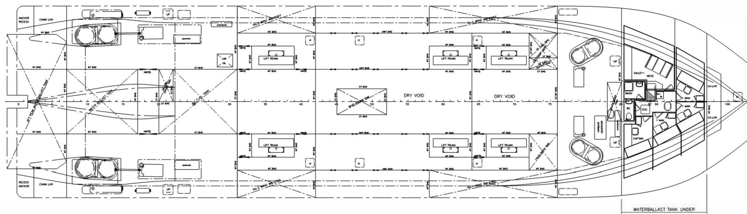
BELOW DECK VIEW
